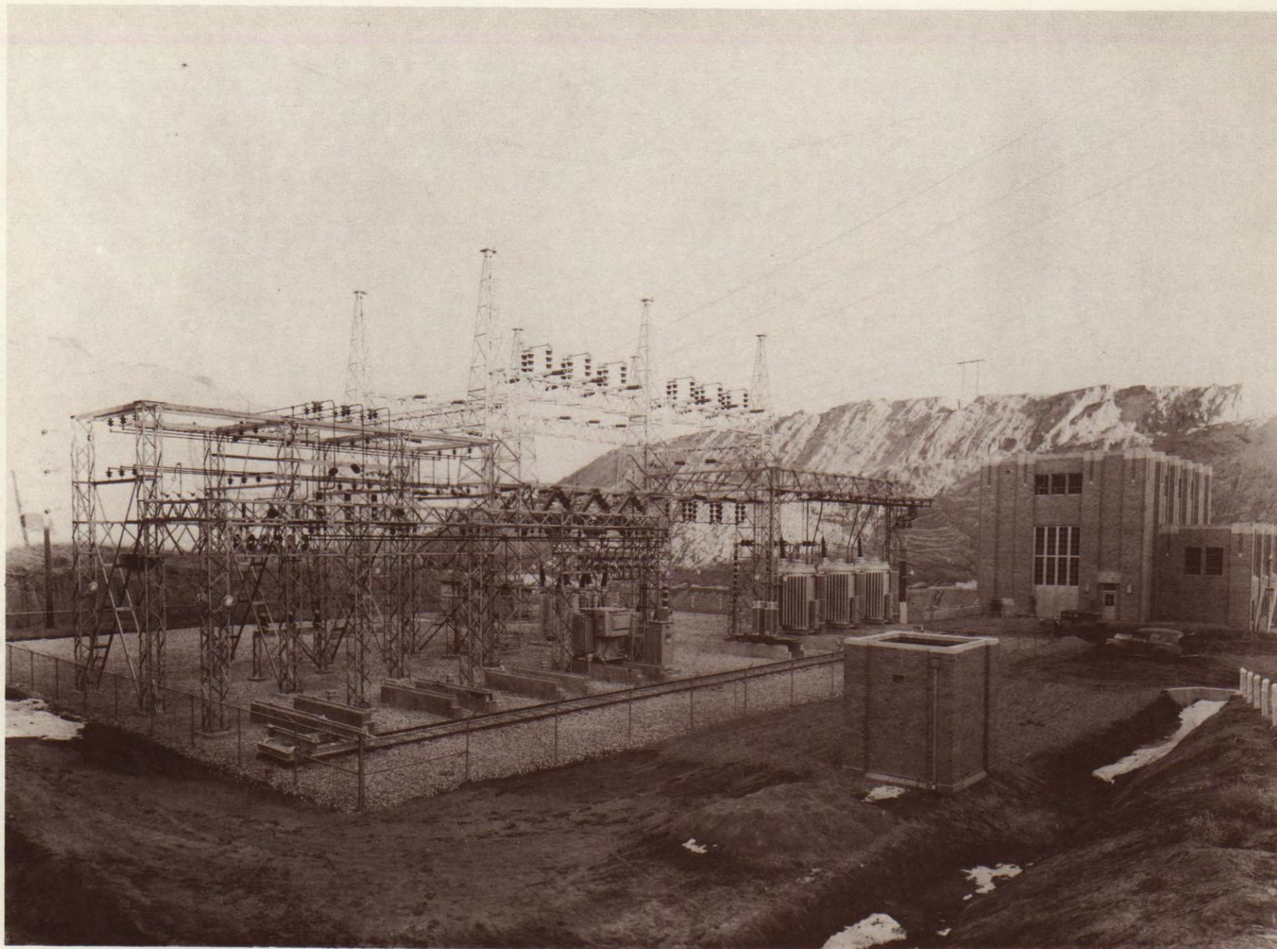
SWITCHYARD AND POWERHOUSE, CENTRAL NEBRASKA PUBLIC POWER AND IRRIGATION DISTRICT Johnson Canyon, Nebraska
