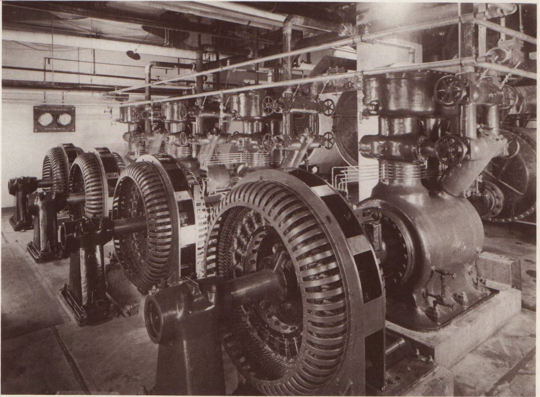
AIRCONDITIONING, INSTALLATION, PHILCADE BUILDING Tulsa, Oklahoma Leon B. Senter, Architect
