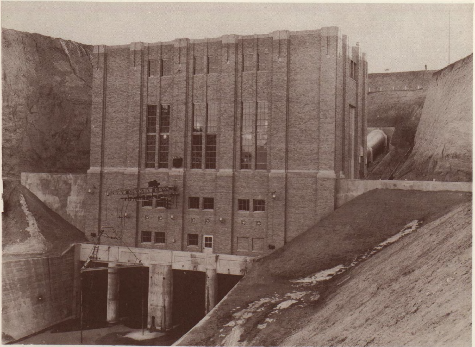
HYDROELECTRIC POWERHOUSE, CENTRAL NEBRASKA PUBLIC POWER AND IRRIGATION DISTRICT Johnson Canyon, Nebraska
