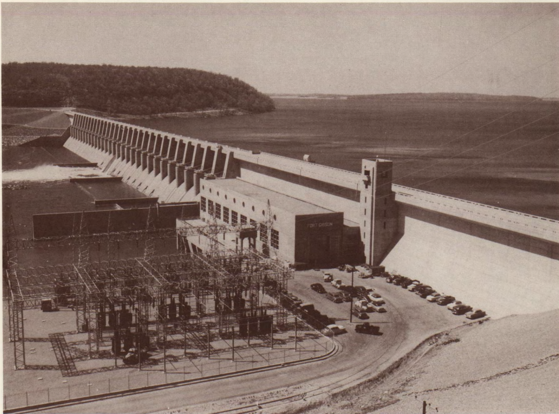
HYDROELECTRIC POWER PLANT AND SWITCHYARD, FORT GIBSON DAM Grand River, Oklahoma
